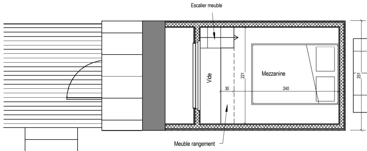
PLAN MEZZANINE
